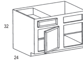
Base Corner - BC42 Center Stile: 6" Blind opening = 15"
