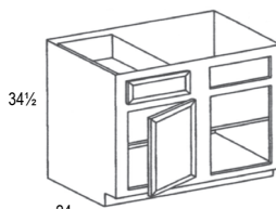
Base Corner - BC39 Center Stile: 6" Blind opening = 12"
