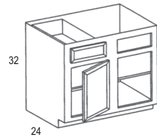
Base Corner - BC36 Center Stile: 6" Blind opening = 9"
