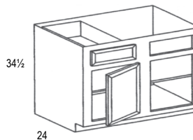
Base Corner - BC42 Center Stile: 6" Blind opening = 15"
