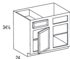
Base Corner - BC36 Center Stile: 6" Blind opening = 9"
